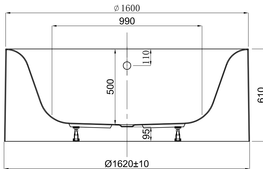
Cross Section D-D
