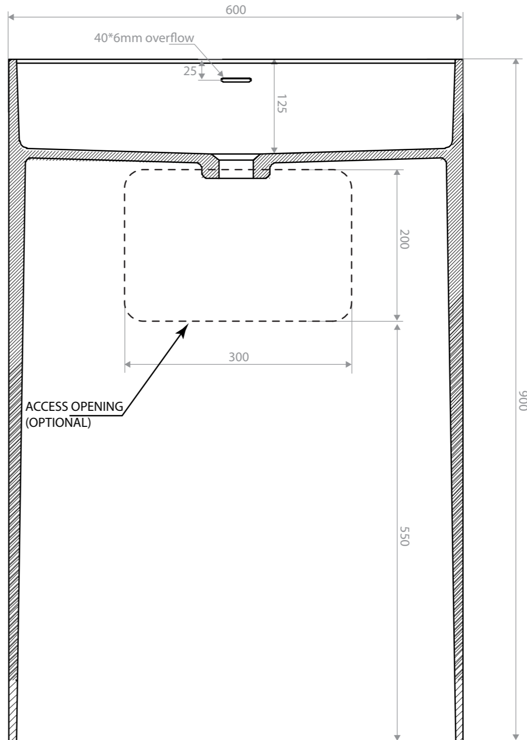
CROSS SECTION VIEW
